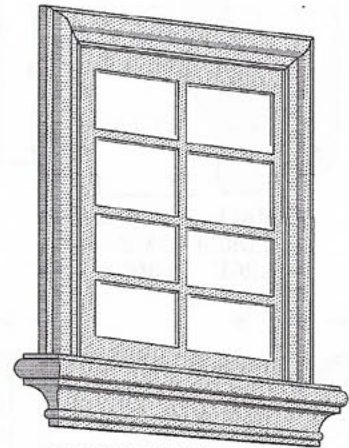
EXAMPLE OF WINDOW SURROUND PFT171S WINDOW TRIM ALONE (TOP) AND WITH PFS517S SILL
